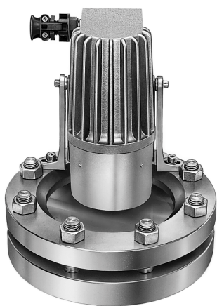
Type PEL 50 deH X2 B, 230 V, 50 W, Ex d e IIC T4 Gb, Ex t IIIC T130°C Db IP67, Ex II 2 G + D, with anti-dazzle shield "B", on circular sightglass to DIN 28120, DN 150, in version "view and light trough one assembly"
