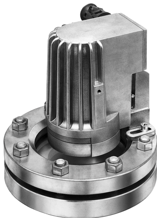
Type PEL 50 deHSch, Ex d e IIC T4 Gb, Ex t IIIC T130°C Db IP67, Ex II 2 G + D, 230 V, 50 W, mounted on circular sightglass to DIN 28120, DN 125, PN 10, in 2 port version.
